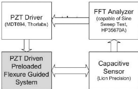
Fig. 5 Experimental setup
