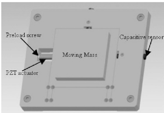
Fig. 1 Schema showing a nano-positioning system which use a flexure guide, a PZT actuator and a capacitive sensor
