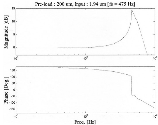
Fig. 18 Response/input relation for a preload of 200 \mu\text{m} and an input amplitude of 1.94 \mu\text{m}
