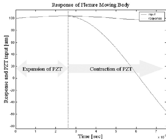
Fig. 15 Response of the moving body, explaining the separation frequency
