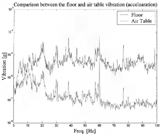
Fig. 24 Comparison between the floor and the air table vibration. Approximately, one order of the floor vibration is decreased by the passive air table
