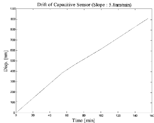
Fig. 26 Drift of the capacitive sensor. The slop of the drift is 5.8 nm/min
