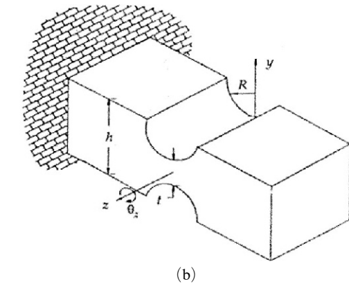
Fig. 2 Simple linear spring : (a) Notch type hinge and (b) Four-bar linkage type motion guide. (Smith, 2000)
