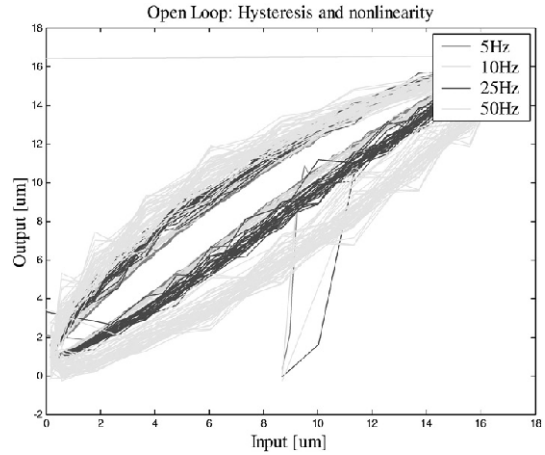
Fig. 8 Hysteresis and nonlinearity of the PZT actuator at various frequencies. As the input frequency increase, the magnitude of the hysteresis increase
